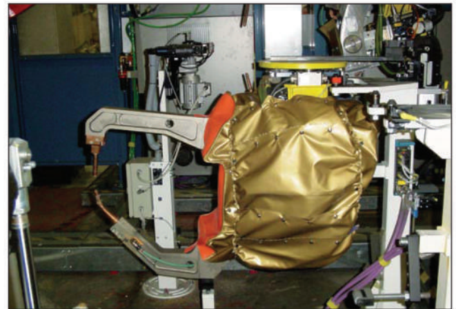
"X" welding gun with switching system
